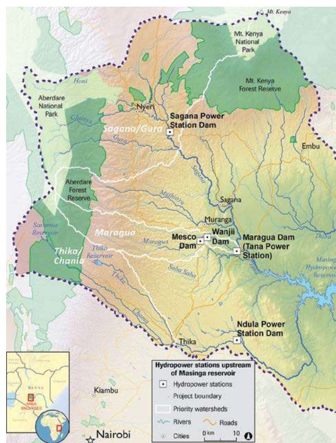
Figure 4 Major water supply and hydropower infrastructure in the Upper Tana
